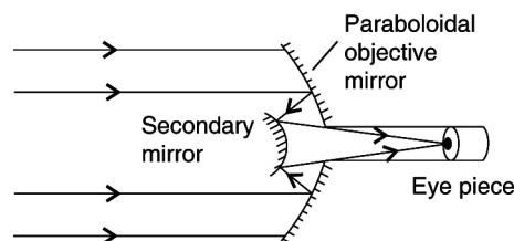
Cassegrain reflecting type telescope
